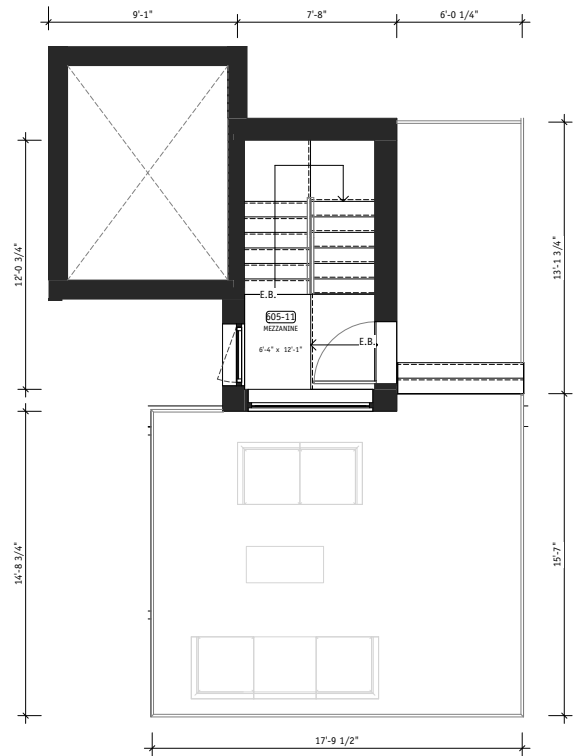
2 PLAN 605 - MEZZ A182 1/4" = 1'-0"
